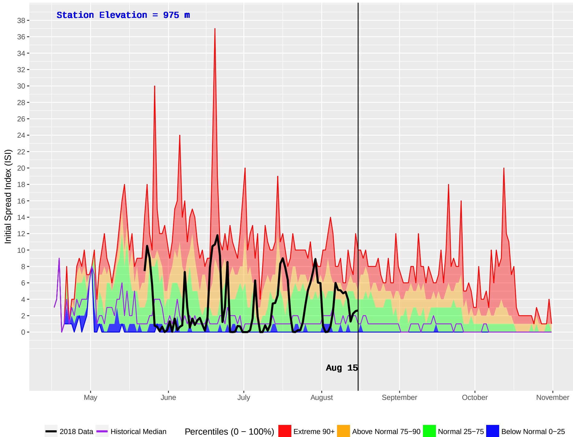
MCGREGOR 2 (192) : Historical (1986–2016) and Current (2018) Daily Initial Spread Index (ISI)
