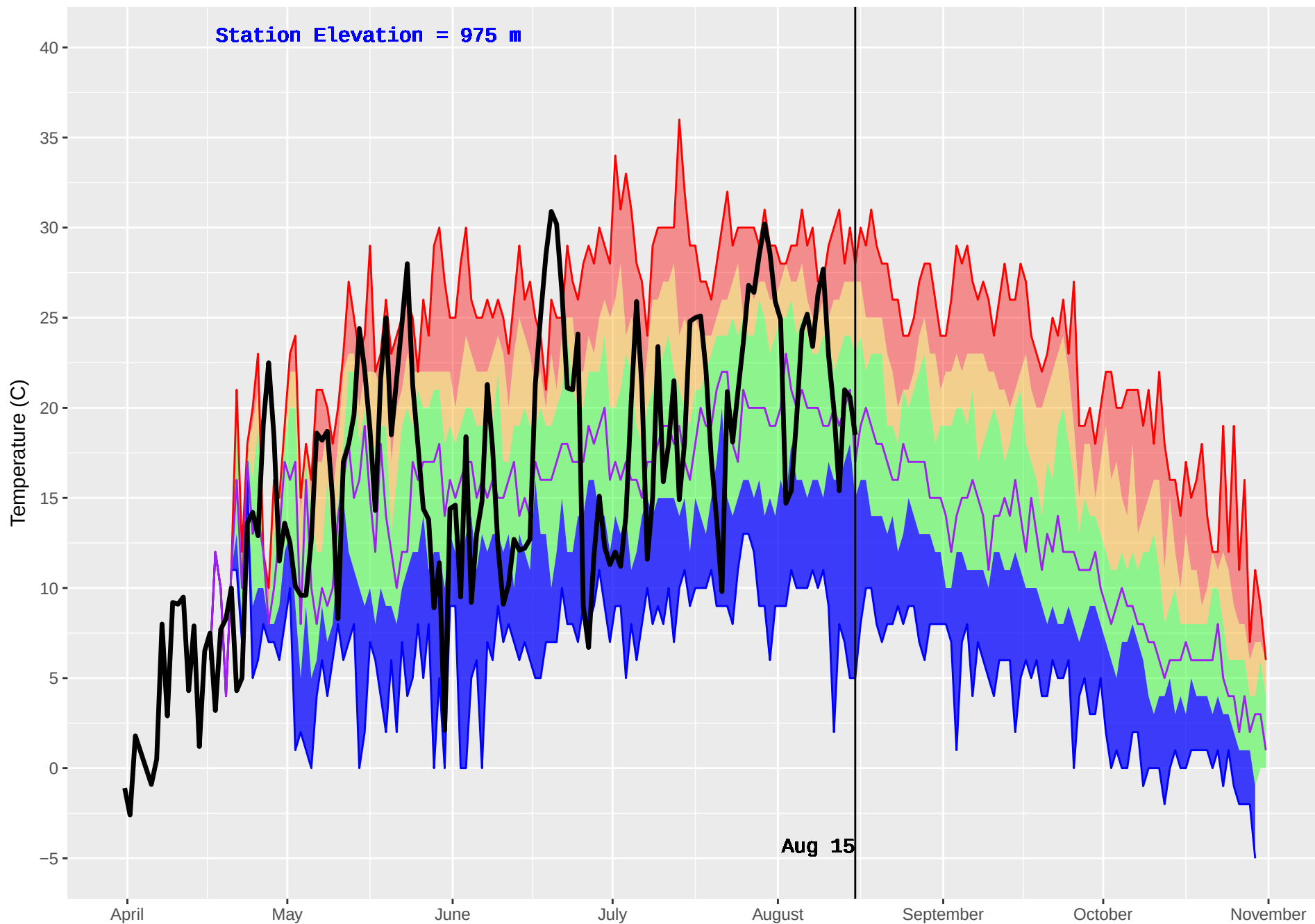
MCGREGOR 2 (192) : Historical (1986–2016) and Current (2018) Daily Temperature
